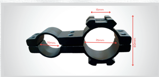
Scope Torch Mount Small
