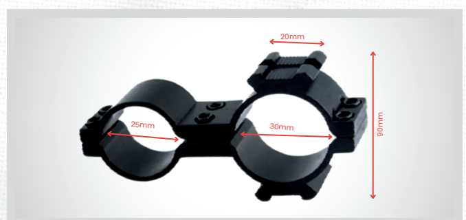
Scope Torch Mount Big
